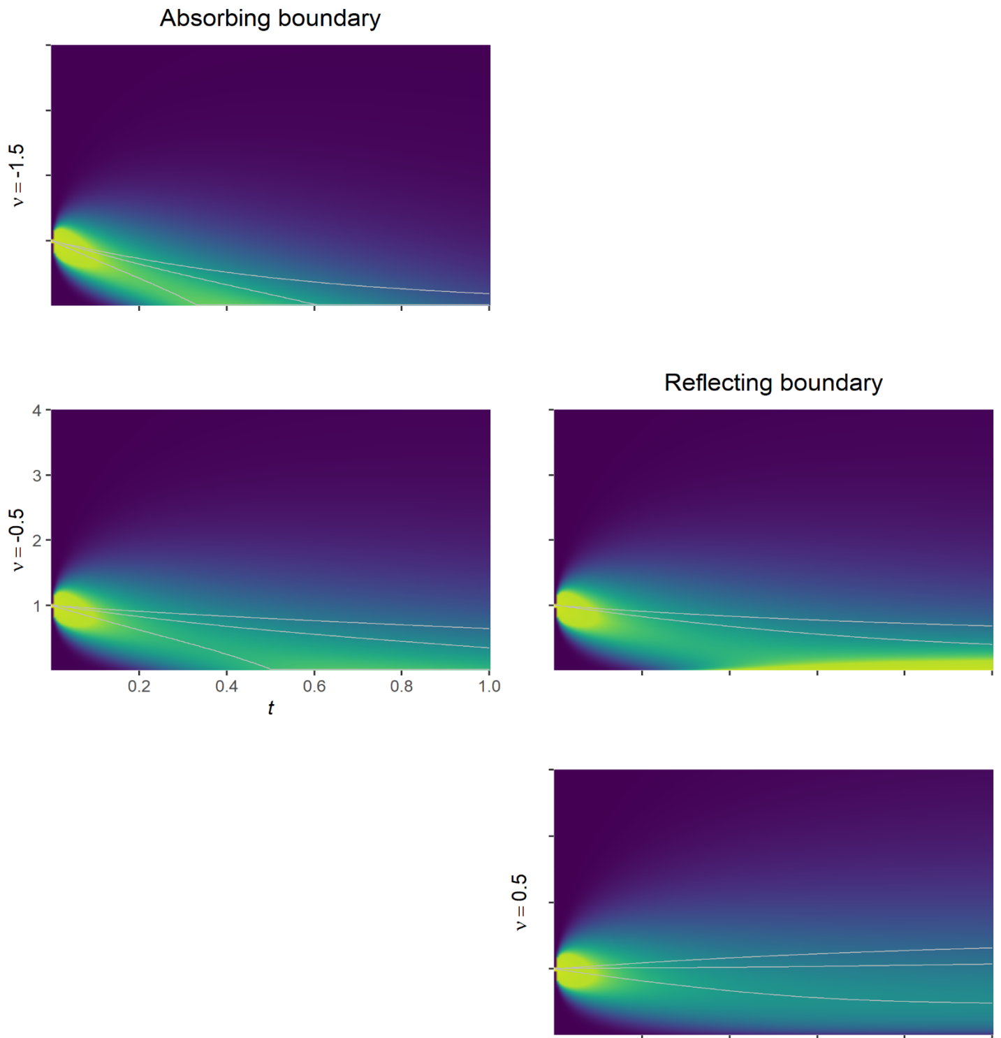
Figure 5. Feller/CIR diffusion f_{\pm\chi^2}^*(X_t; X_0, t, a, b, \nu) for \nu = -1.5, -0.5, +0.5 , with X_0 = a = 1, b = -1
